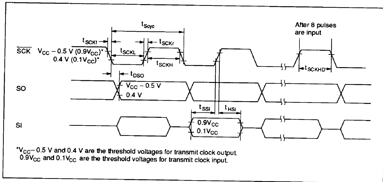
Figure 56 Timing of Serial Interface
