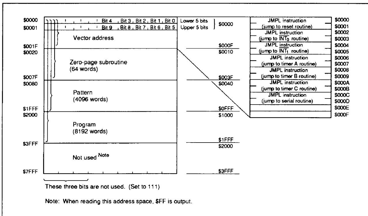
Figure 36 PROM Mode Function Diagram
