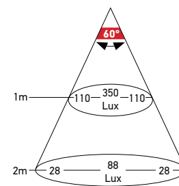
5000 K - 20 LED
