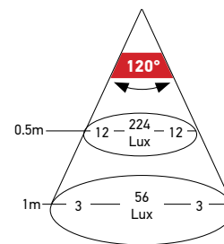
5000 K - 12 LED
