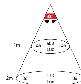
5000 K - 36 LED
