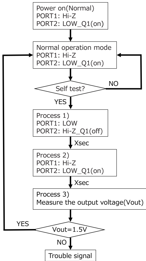
Figure 4 - Self-diagnosis flow chart
