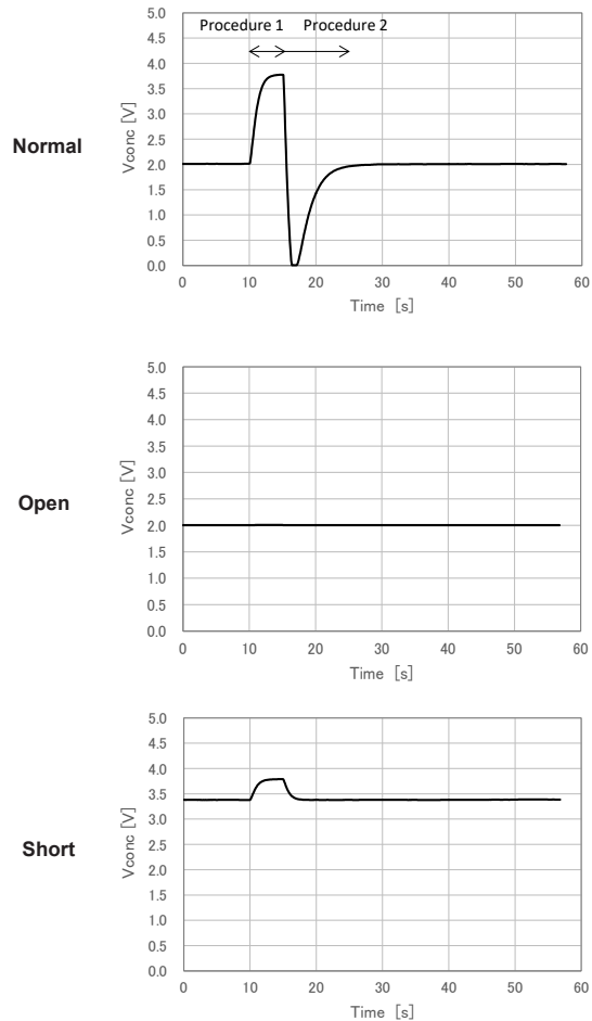
Figure 5 - Vout response patterns for self-diagnosis
