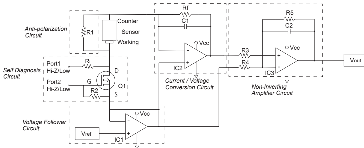
Figure 1 - Example circuit for TGS5xxx sensors
