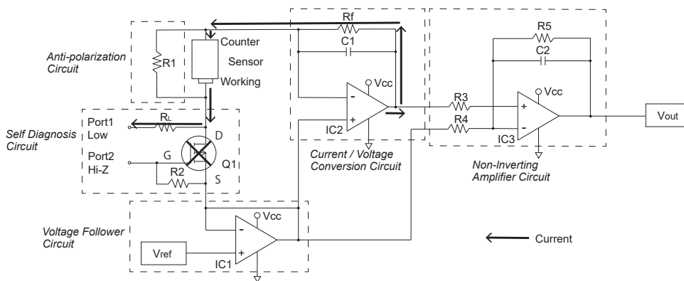
Figure 3 - Self-diagnostic circuit
