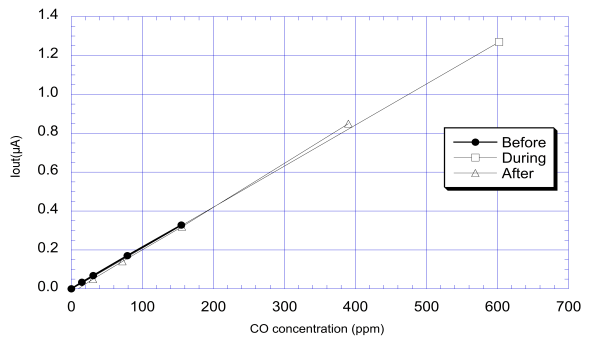
Figure 11b - Normal operation test (20°C/40%RH)
