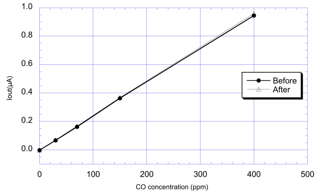
Figure 17b - Effects of shipping and storage
