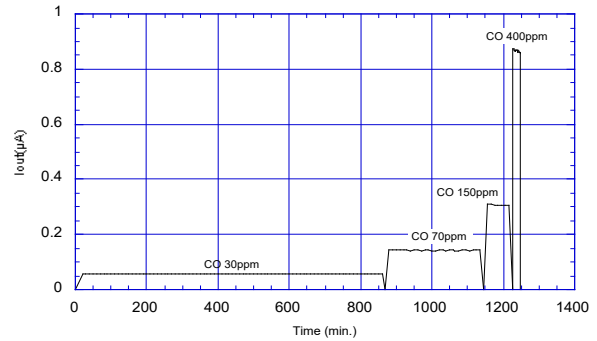
Figure 12a - Sensitivity test (20°C/40%RH)
