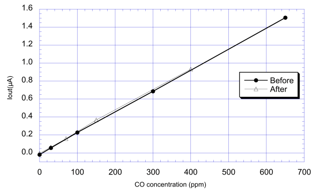
Figure 16 - Durability against corrosion
