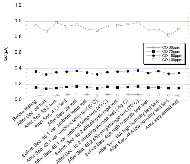
Figure 21 - Sequential test
