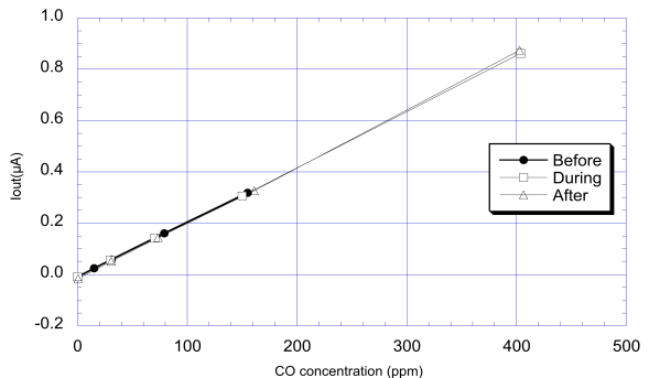
Fig. 12b - Sensitivity test (20°C/40%RH)
