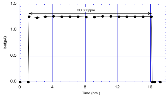
Figure 11a - Normal operation test (CO 600±30ppm for 12 hours at 20°C/40%RH)
