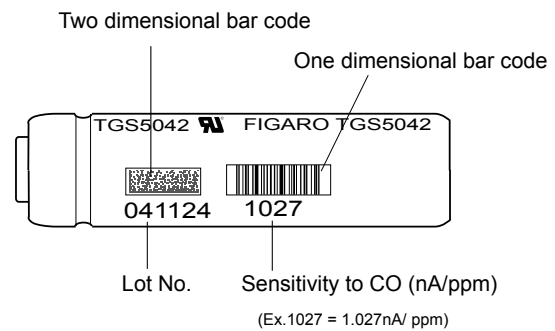
Figure 24 - TGS5042 markings (NOTE: UL Mark may appear on shrink tube)
