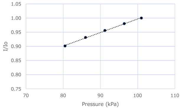
Fig. 13 - Pressure dependency
