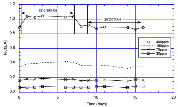
Figure 18a - Humidity test
