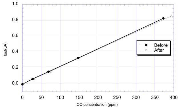
Figure 19 - False alarm test
