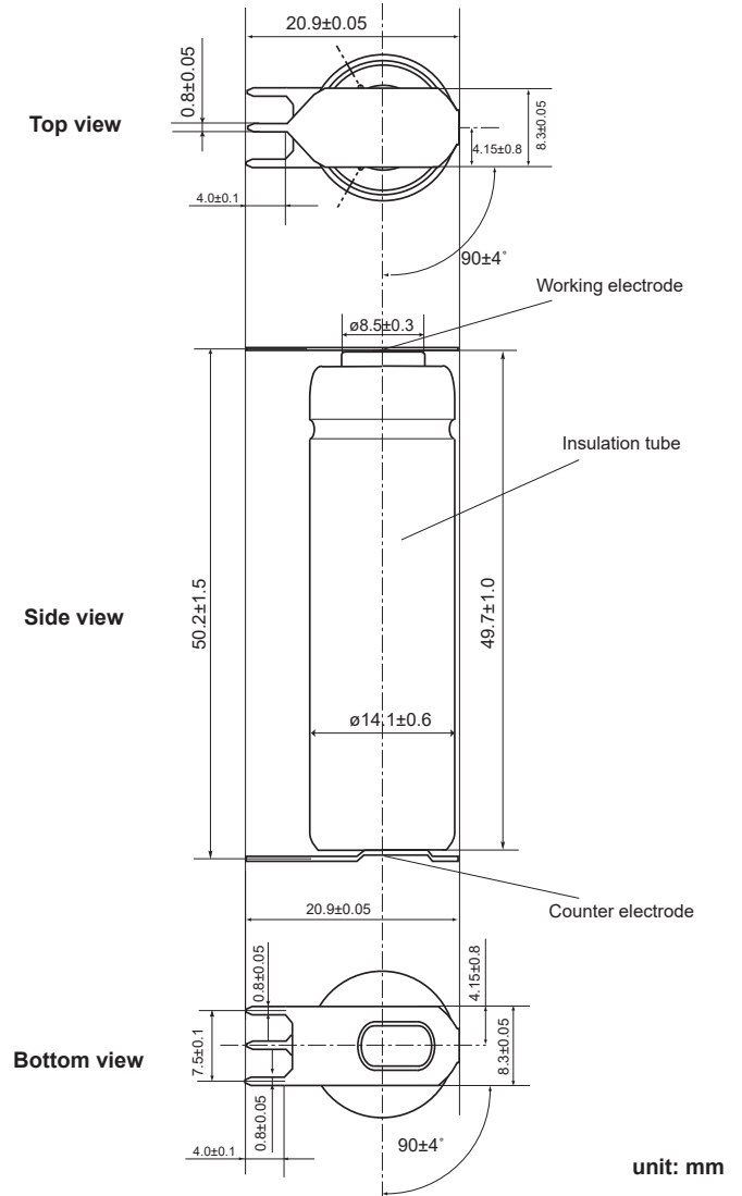
Figure 25 - TGS5042 Dimensions (lead configuration)
