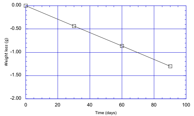
Figure 23 - Water loss test
