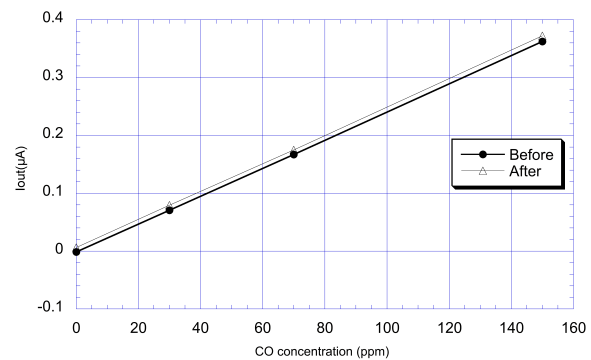
Figure 14b - Interference gas test (20°C/40%RH)
