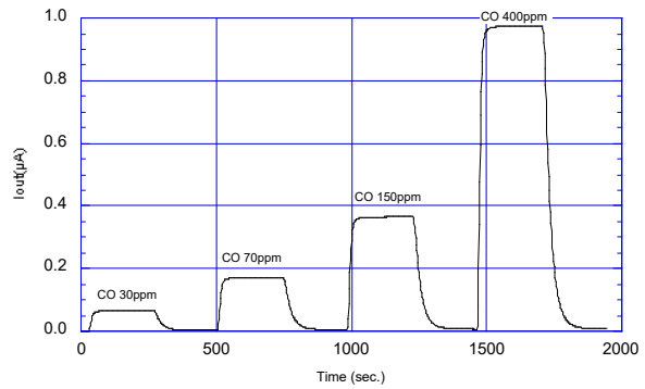
Figure 8 - Response pattern
