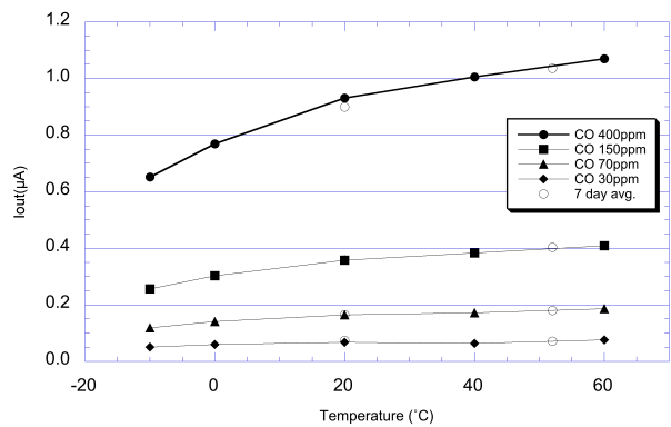
Figure 18b - Humidity test (all data at 50%RH except Sec. 46A test points)
