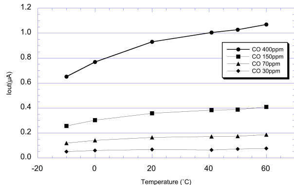
Figure 17a - Operation in high and low temperature (all data at 50%RH except Sec. 45.1 test points)
