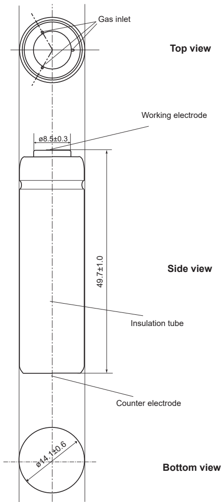
Figure 3 - Dimensions
