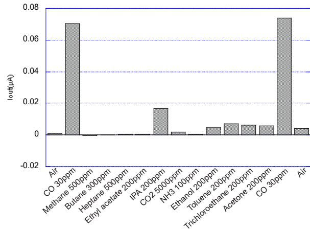
Figure 14a - Interference gas test (20°C/40%RH)
